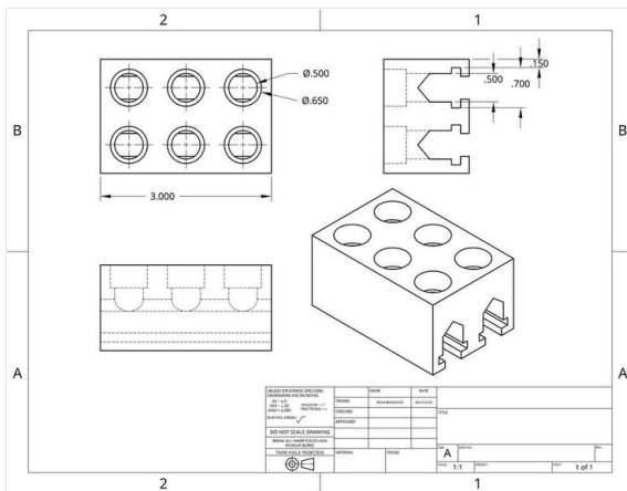
Pin-guide block. 3.000 in wide manifold with six bores ( \varnothing .500 in through, \varnothing .650 in counterbore) carrying the dome pins, and snap-fit tabs (.150/.500/.700 in) that key it to the enclosure.
