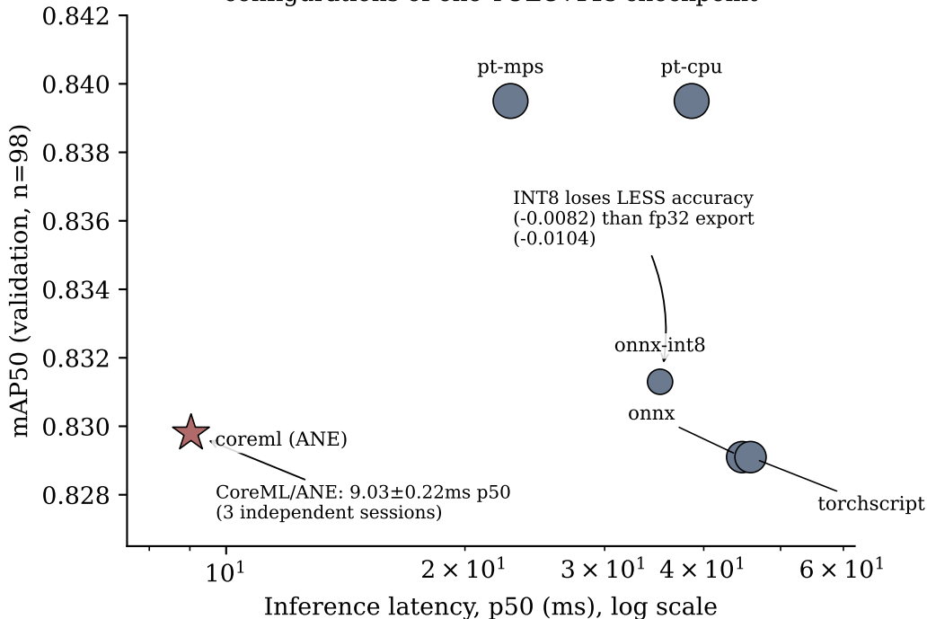
Latency-accuracy tradeoff across six export configurations of one YOLOv11s checkpoint
