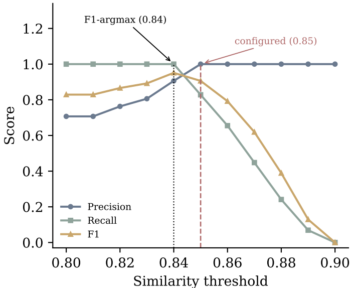
RAG threshold sweep (29 pos. / 12 hard-neg. queries)
