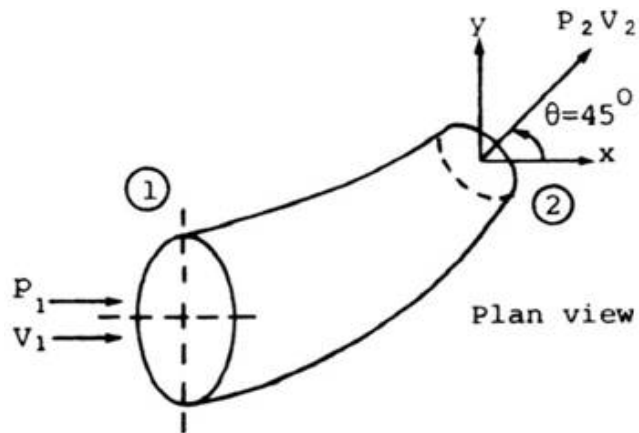
Figure 3. Flow through a 45° pipe bend.
