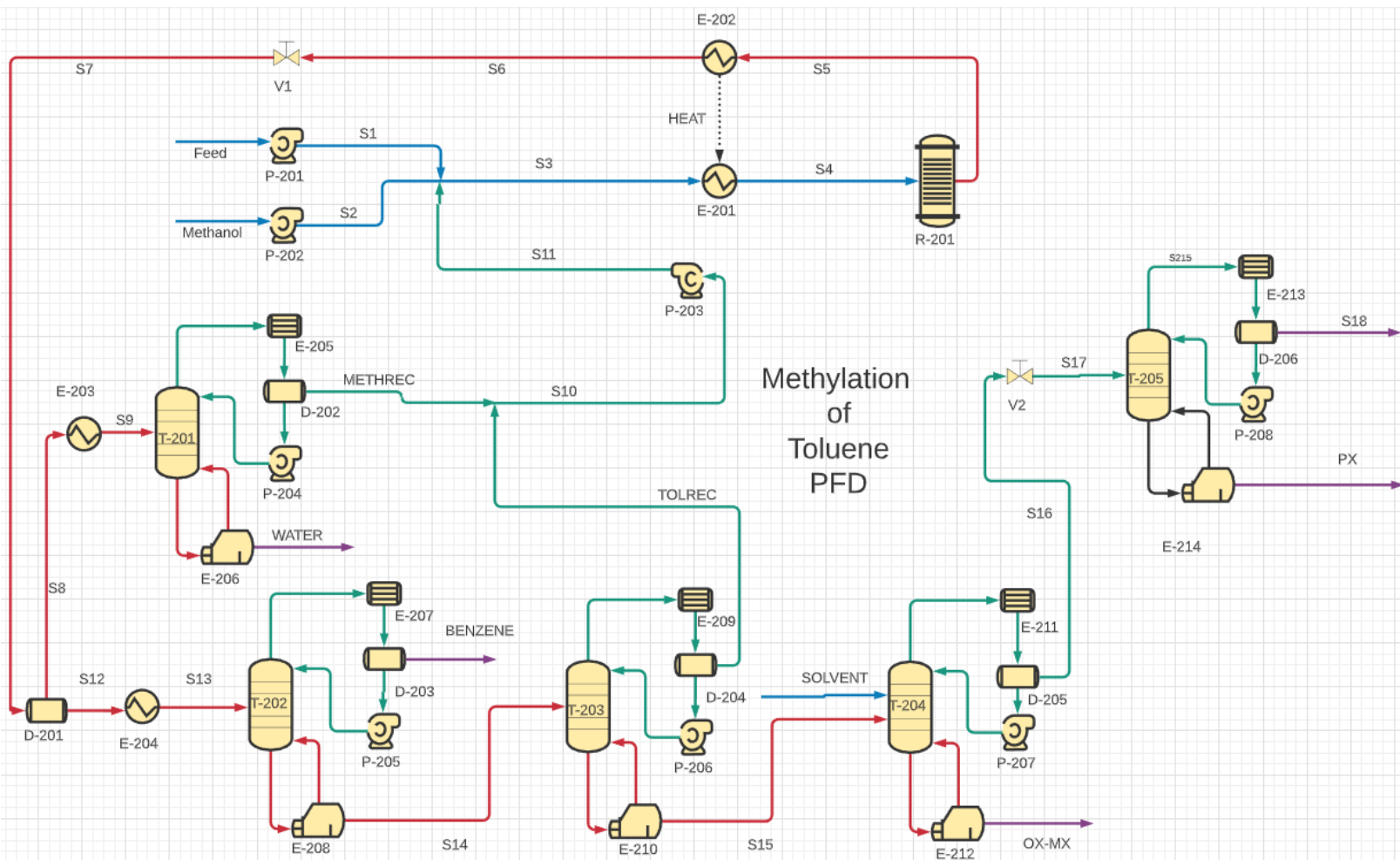
Figure A3-1: Finalized PFD of para-xylene production through the methylation of toluene
