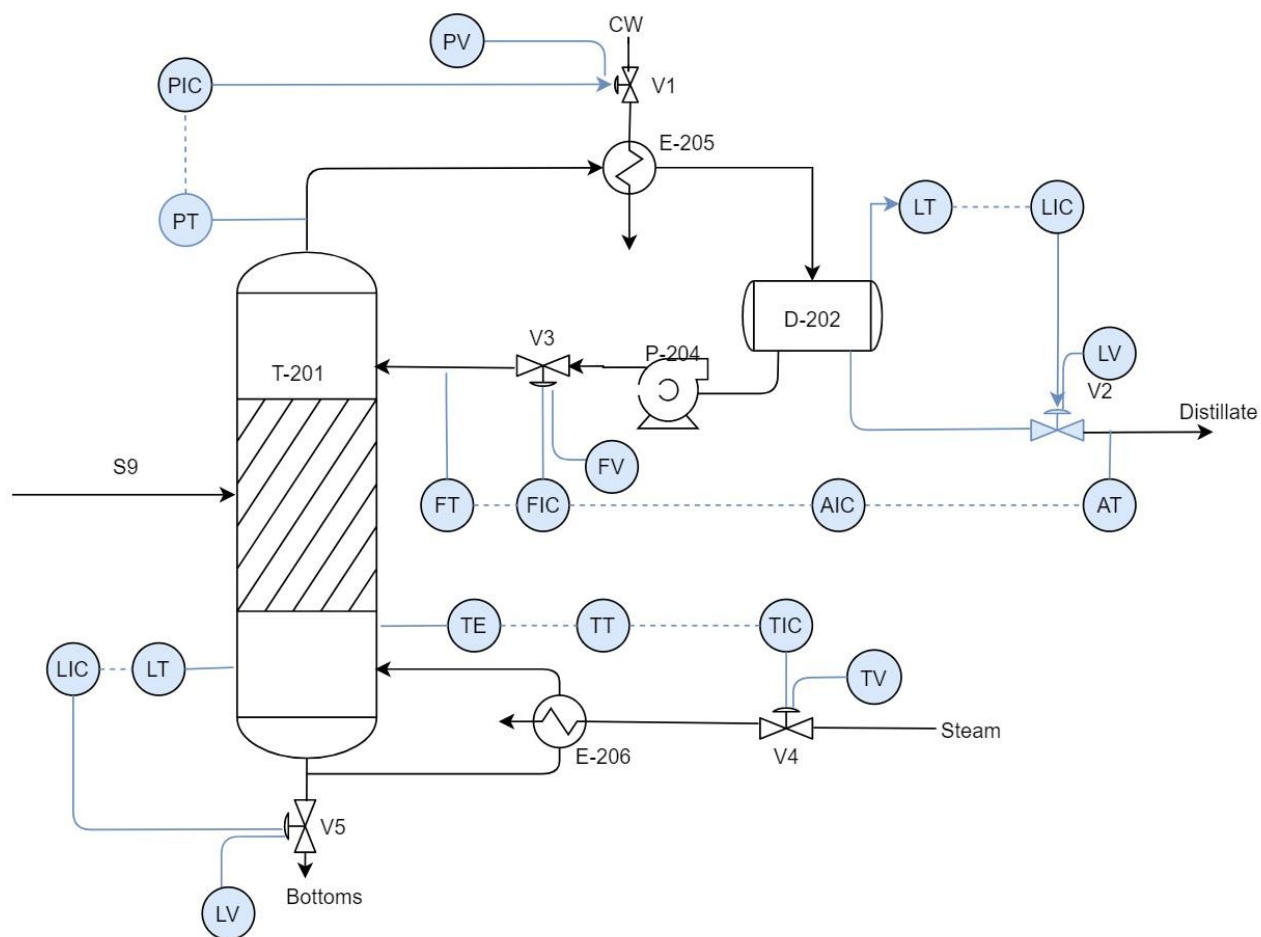
Figure 8: Methanol Distillation column (T-201) control scheme Before HAZOP
