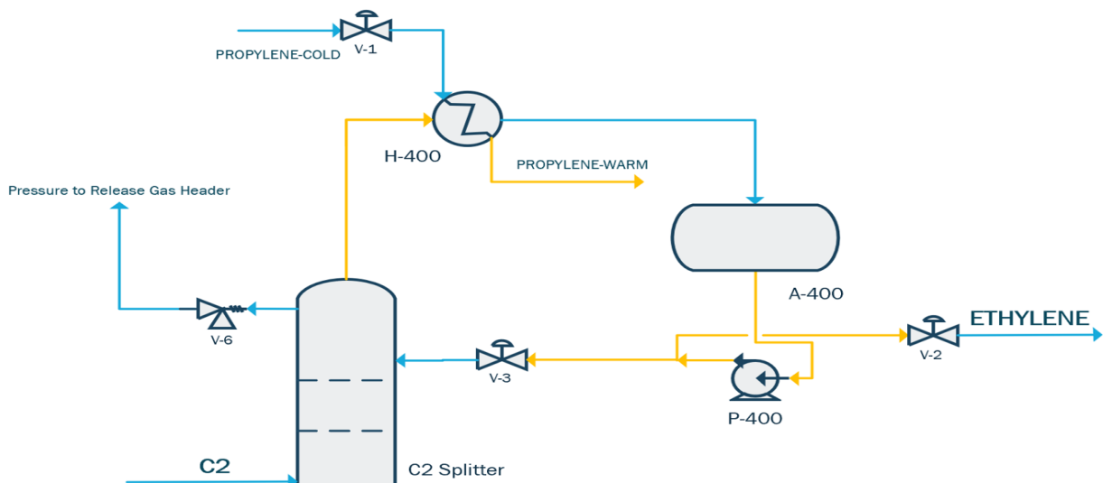
Figure 15: Tops Before HAZOP
