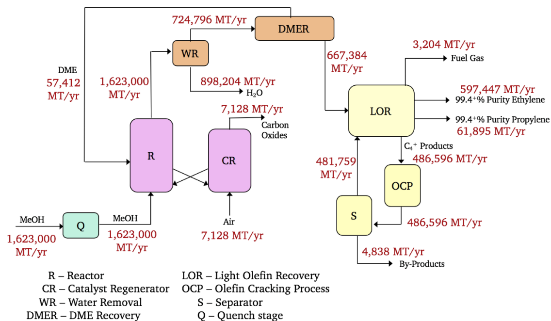
Figure 23: BFD of UOP's Advanced MTO Process [12]
