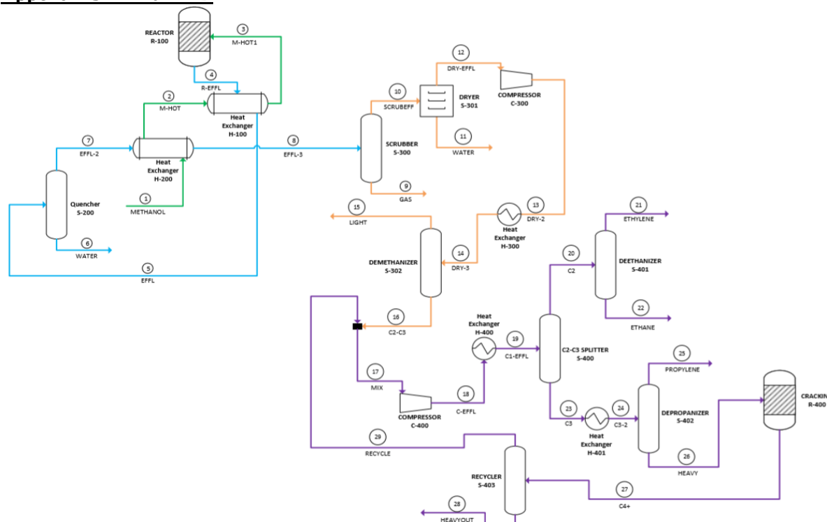
Figure 24: Advanced MTO Preliminary PFD [10]
