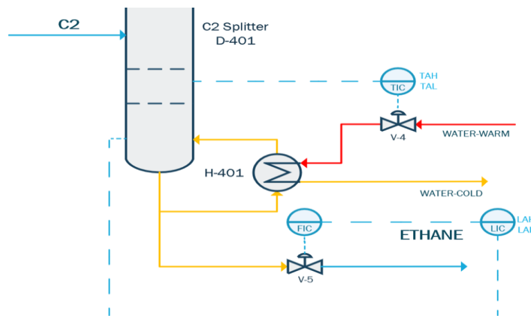
Figure 17: Bottoms After HAZOP
