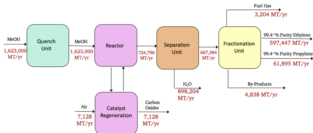
Figure 22: Simplified BFD of UOP's Advanced MTO Process
