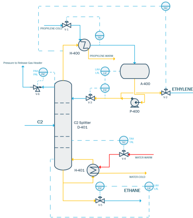
Figure 16: C2 Splitter Overview After HAZOP
