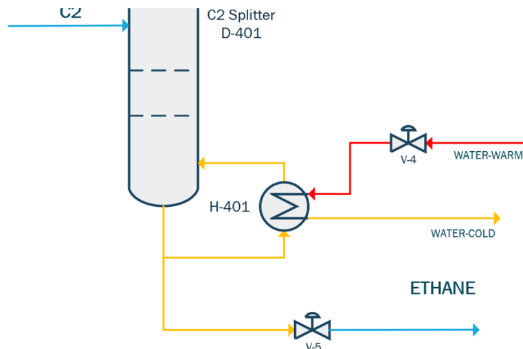
Figure 14: Bottoms Before HAZOP
