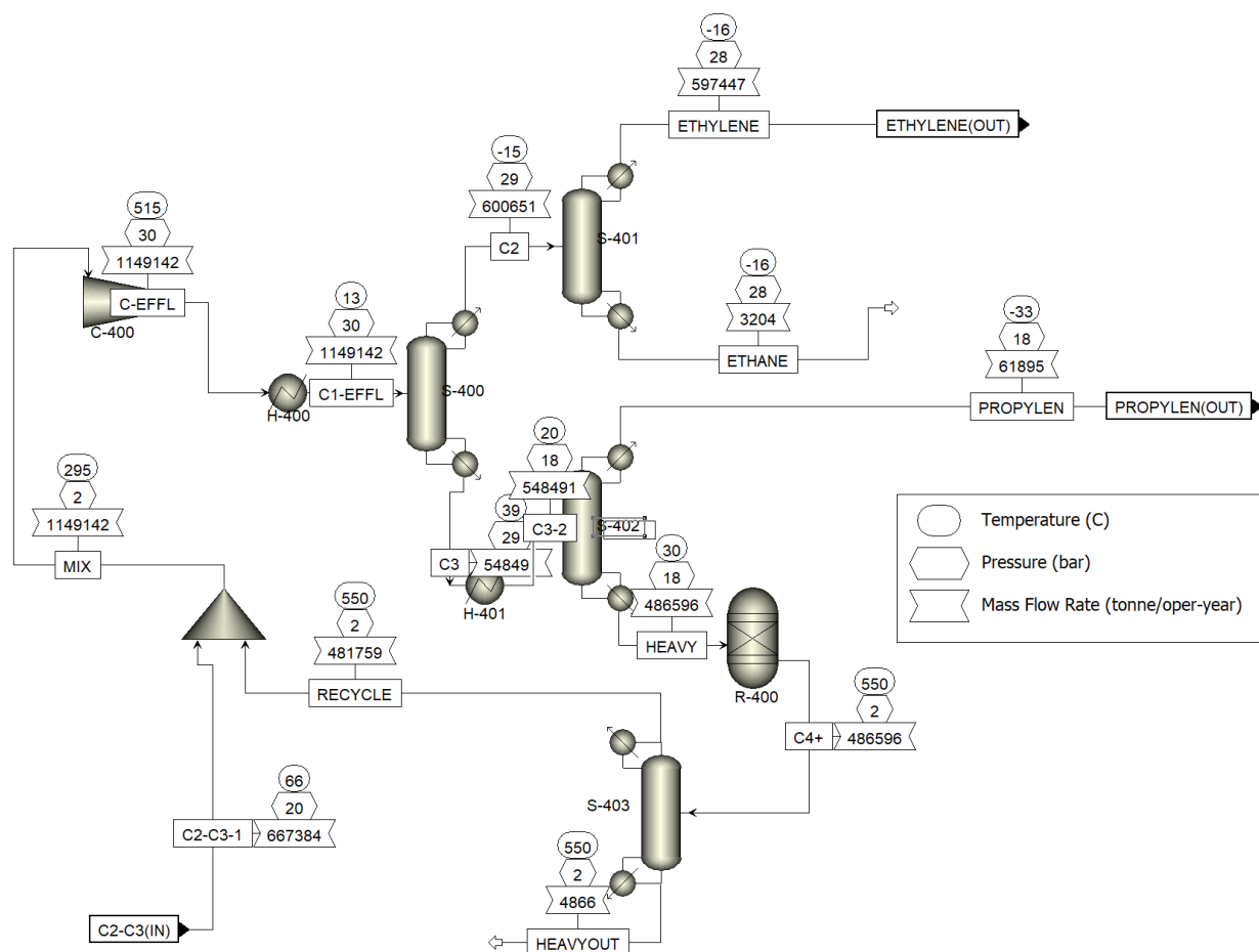
Figure 29: Sep PFD
