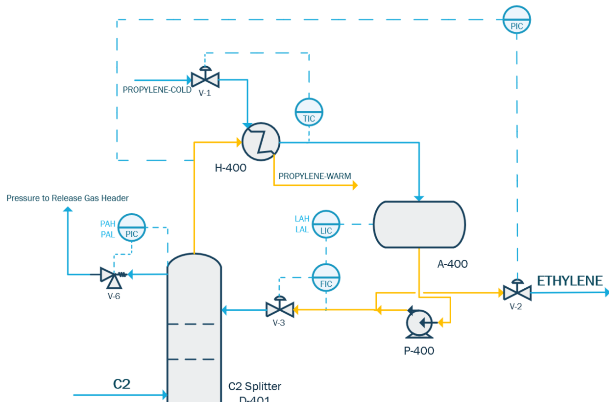
Figure 18: Tops After HAZOP
