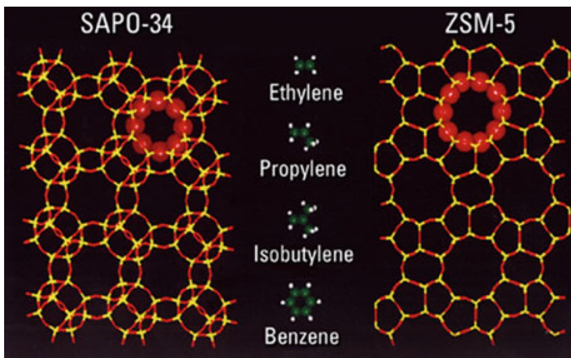
Figure 8: SAPO-34 and ZSM-5 Catalyst Comparison [20]
