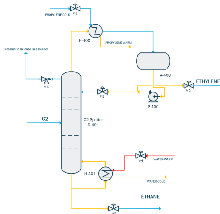
Figure 13: C2 Splitter Overview before HAZOP
