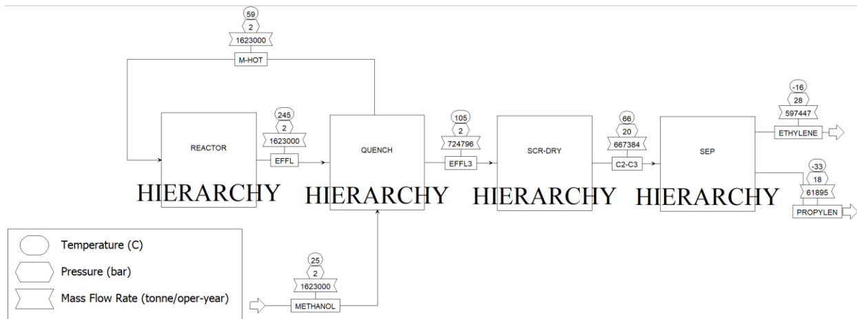
Figure 25: Aspen MTO PFD
