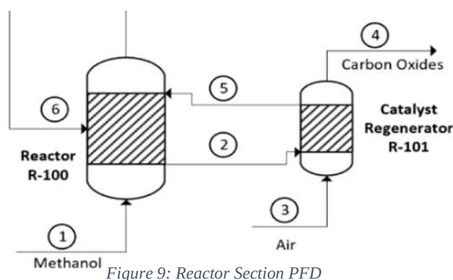
Figure 9: Reactor Section PFD
