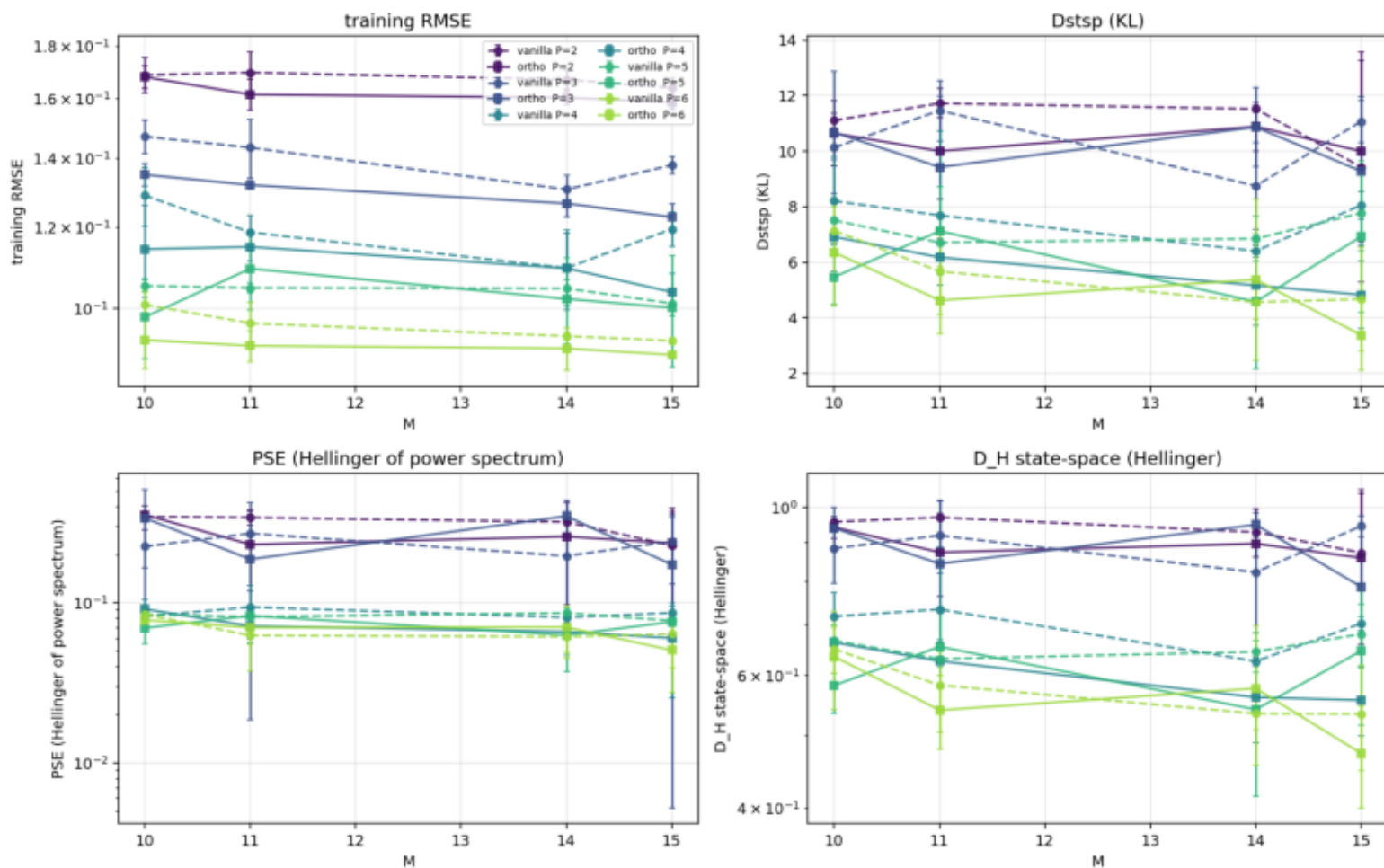
Metrics vs M, mean +/- std over 3 seeds (vanilla dashed, ortho solid)
