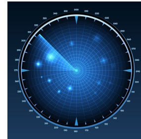
Dataset 2: Sonar
