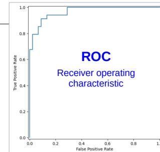
Diagnostic plots
