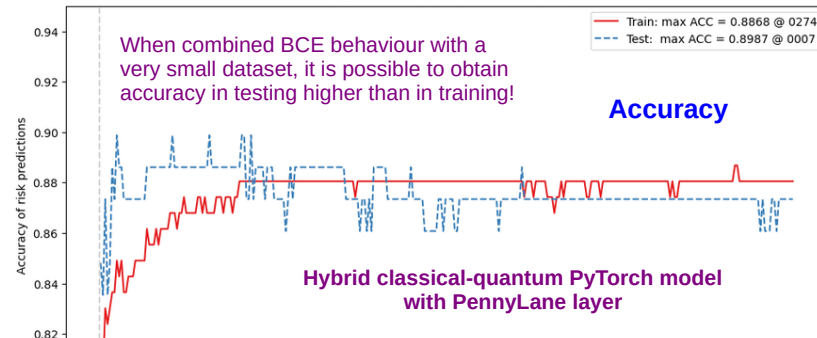
Classification of car insurance risk
