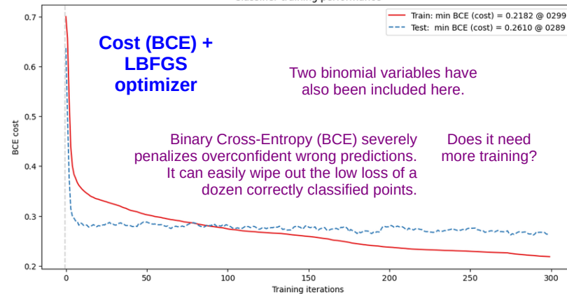
Classifier training performance
