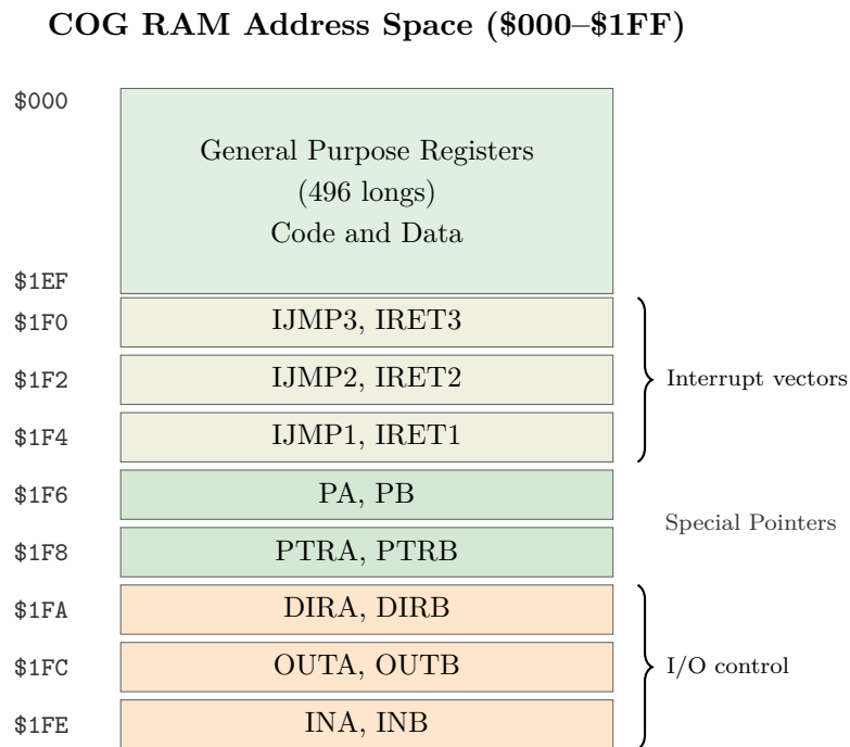
Figure 1.2: COG Memory Map
