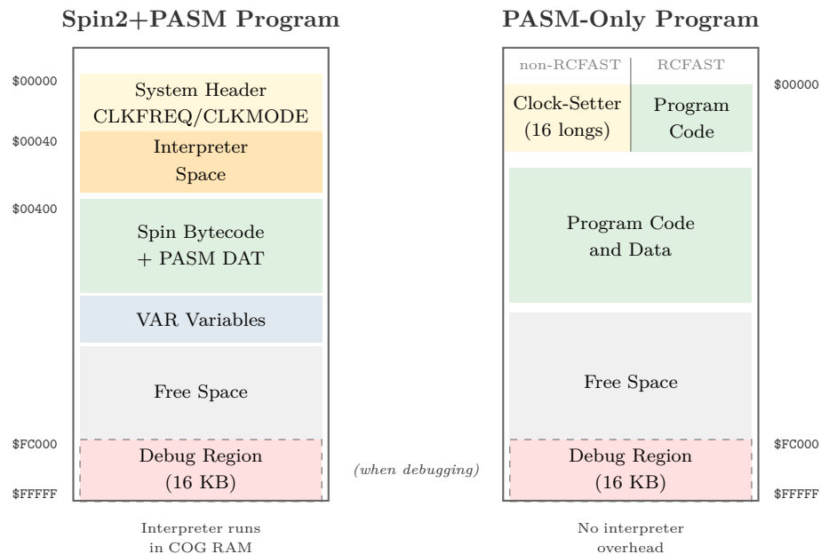
Figure 1.5: Hub Memory Layout: Spin2+PASM vs PASM-Only Programs
