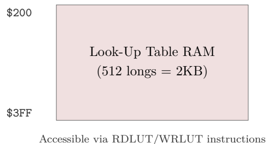
Figure 1.3: LUT Memory Map
