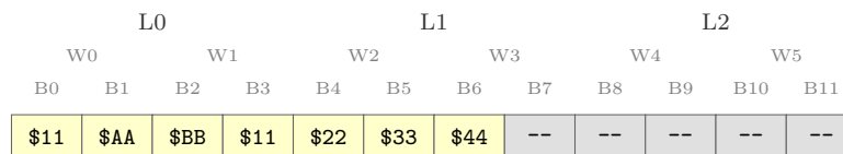
Figure D.3: Memory Layout Before ALIGNW
