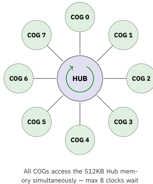
Figure 4.1. Figure 4.1: Hub Access Rotation (“Egg Beater”)
