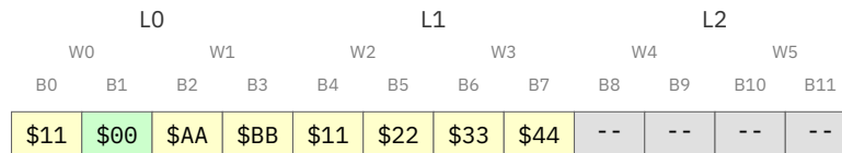
Figure 6.4. Figure D.4: Memory Layout After ALIGNW
