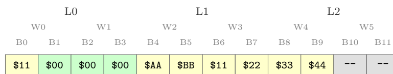
Figure D.2: Memory Layout After ALIGNL
