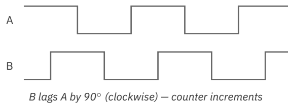
Figure 14.1. Quadrature A/B signals
