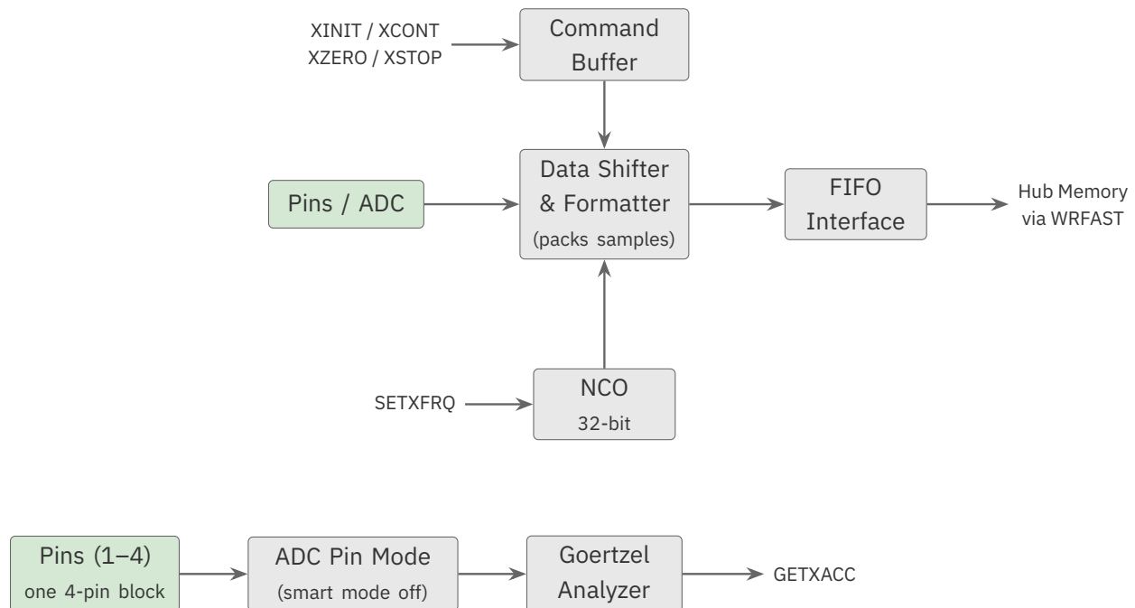
Figure 2.2. Streamer input paths: pins to hub, through the same hub FIFO set up by WRFAST; and the Goertzel analyzer
