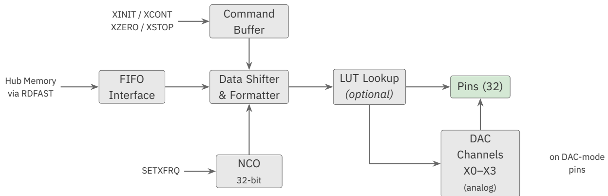
Figure 2.1. Streamer output path: hub to pins, through the cog's hub FIFO set up by RDFAST
