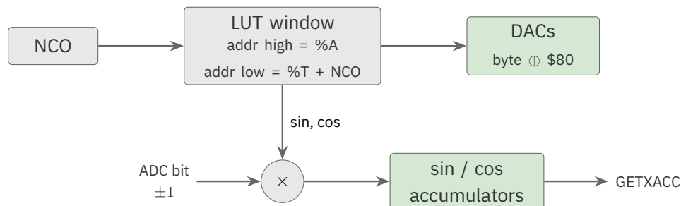
Figure 10.1. DDS output with Goertzel accumulation (every clock). The window is 4 to 512 entries, selected by S[11:9] ; \%A bounds it and \%T offsets playback within it.
