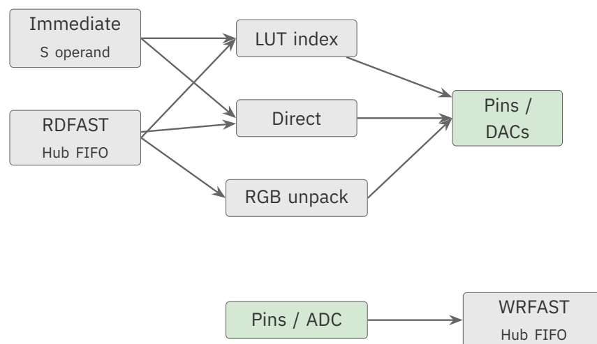
Figure 2.3. Streamer data-flow paths
