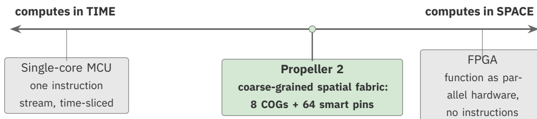
Figure 3.1. Computing in time vs. in space. A single-core microcontroller runs one instruction stream; an FPGA lays function out as parallel hardware. The Propeller 2 sits between them — a coarse-grained spatial fabric you assign function to.
