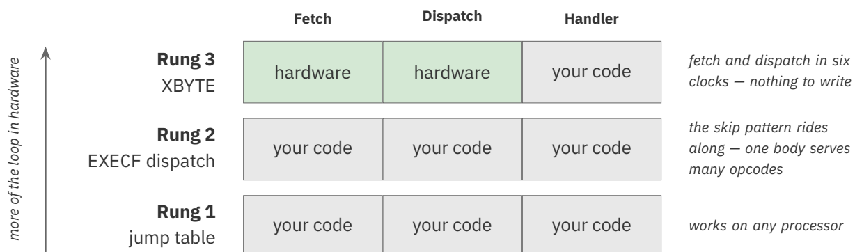
Figure 7.1. The dispatch ladder: each rung moves more of the loop into hardware
