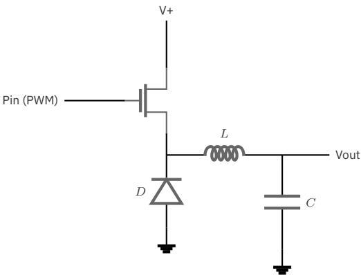
Figure 9.5. Typical SMPS (buck) circuit
