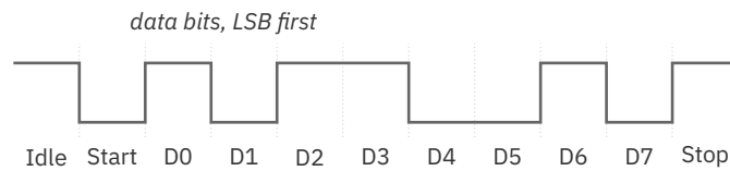
Figure 11.1. UART transmit frame
