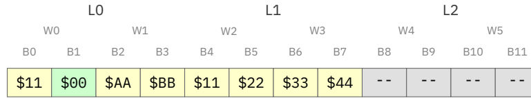
Figure 6.4. Figure D.4: Memory Layout After ALIGNW
