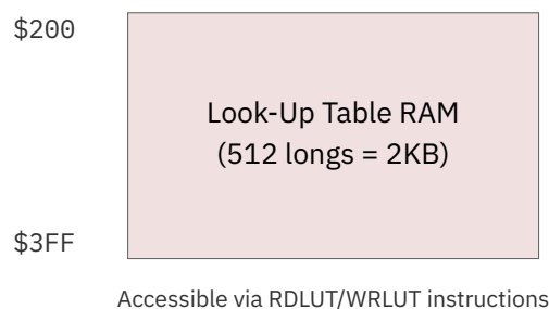
Figure 1.3. Figure 1.3: LUT Memory Map
