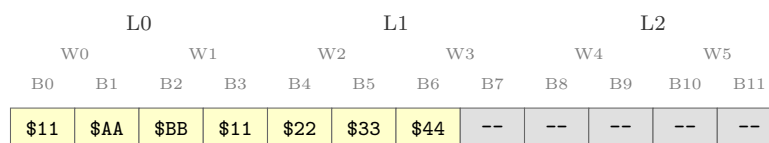
Figure D.1: Memory Layout Before ALIGNL
