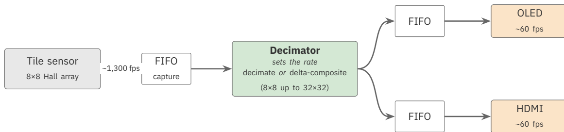
A FIFO at every stage — and the decimator, not the sensor or the displays, sets the rate.
