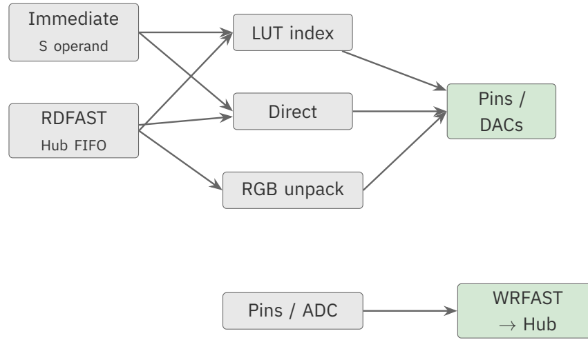
Figure 2.2. Streamer data-flow paths
