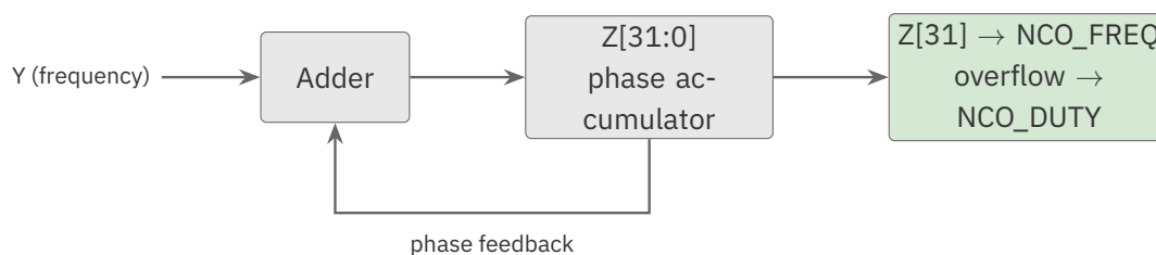
Figure 8.1. NCO architecture
