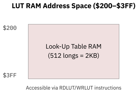
Figure 1.3. Figure 1.3: LUT Memory Map
