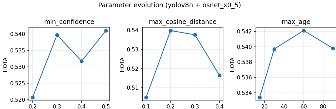
Figure 4: Changing one parameter at a time (yolov8n + osnet_x0_5).
