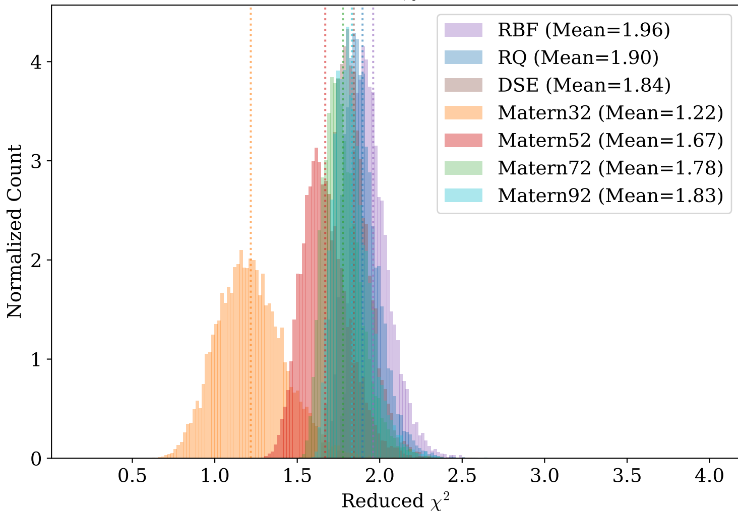
Distribution of Reduced \chi^2 for different Kernels
