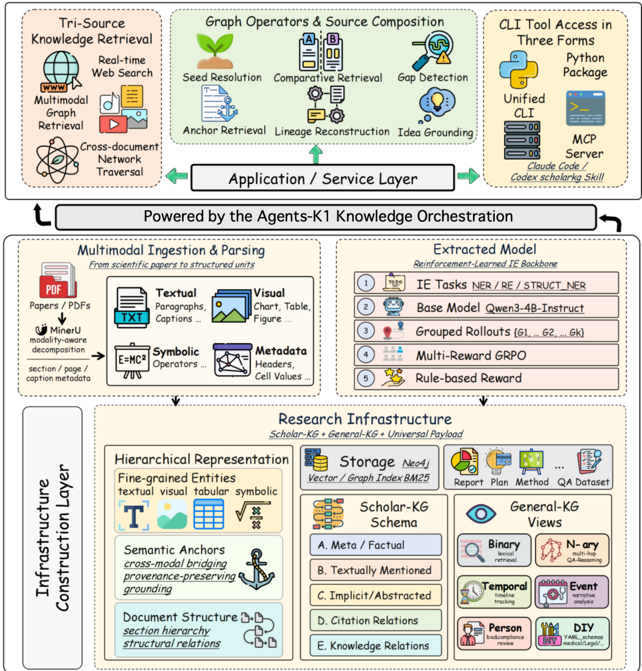
Figure 2 | Overall framework of Agents-K1. Agents-K1 features three parts. The infrastructure construction layer parses multimodal documents into structured knowledge graphs ( Scholar-KG and General-KG ). Utilizing this foundation, the application/service layer offers a tri-source agent CLI as the main interface, enabling comprehensive and auditable research workflows such as comparative analysis and idea grounding.
