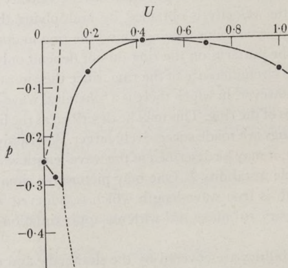
FIGURE 1. Values of \mathcal{R}p (instability or growth rate), and |\mathcal{J}p| (radian frequency of oscillation), related to wave-length 2\pi U^{-\frac{1}{2}} as in the relation (8.3) with I = 0 . This is a case of stationary waves with finite wave-length. Full line, \mathcal{R}p ; broken line, -|\mathcal{J}p| (zero for U > 0.071 ); dotted line, \mathcal{R}p' . The full circles on the curve for \mathcal{R}p indicate the values of U, p actually achievable on the finite ring considered in §10, with s = 0 on the extreme left, s = 5 on the right.
