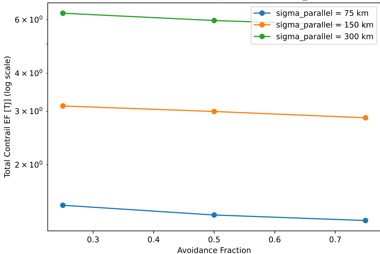
EF vs Avoidance Fraction, by ISSR Size (climb_500m)
