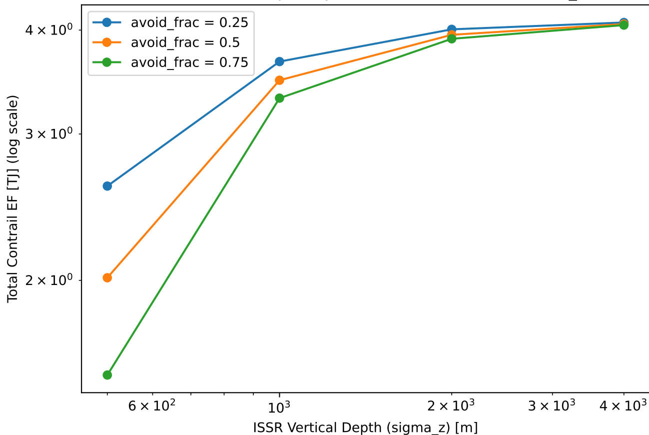
EF vs ISSR Vertical Depth, by Avoidance Fraction (descend_500m)
