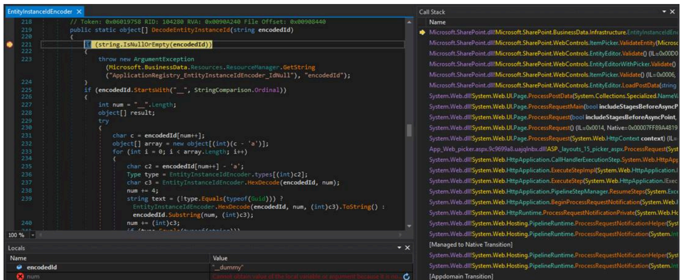
Figure 7: Break point at *EntityInstanceIdEncoder.DecodeEntityInstanceId(string) *with the encodedId value "__dummy"
