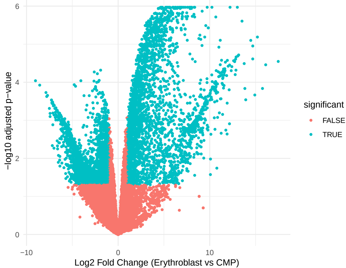
limma-voom Volcano Plot
