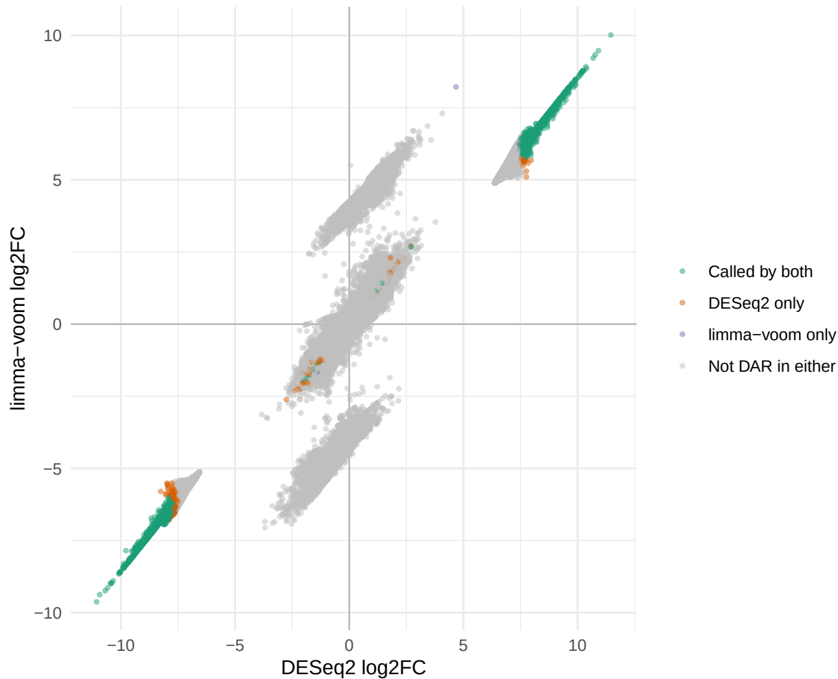
ATAC DESeq2 vs limma-voom Concordance ( r = 0.870 )
