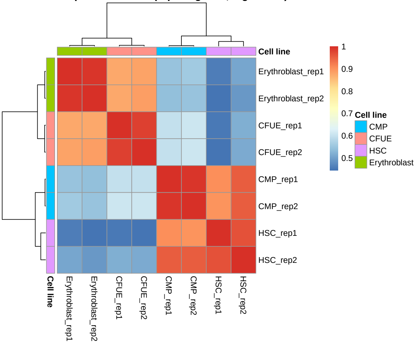
RNA Sample Correlation (top DE genes, log2 scale)
