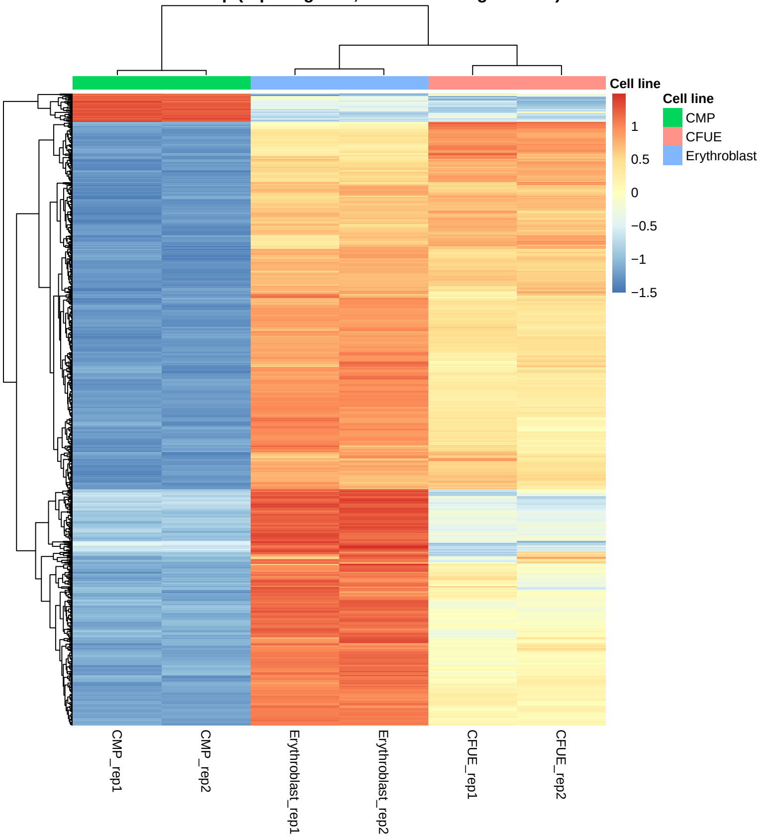
RNA Heatmap (top DE genes, row-scaled log2 values)
