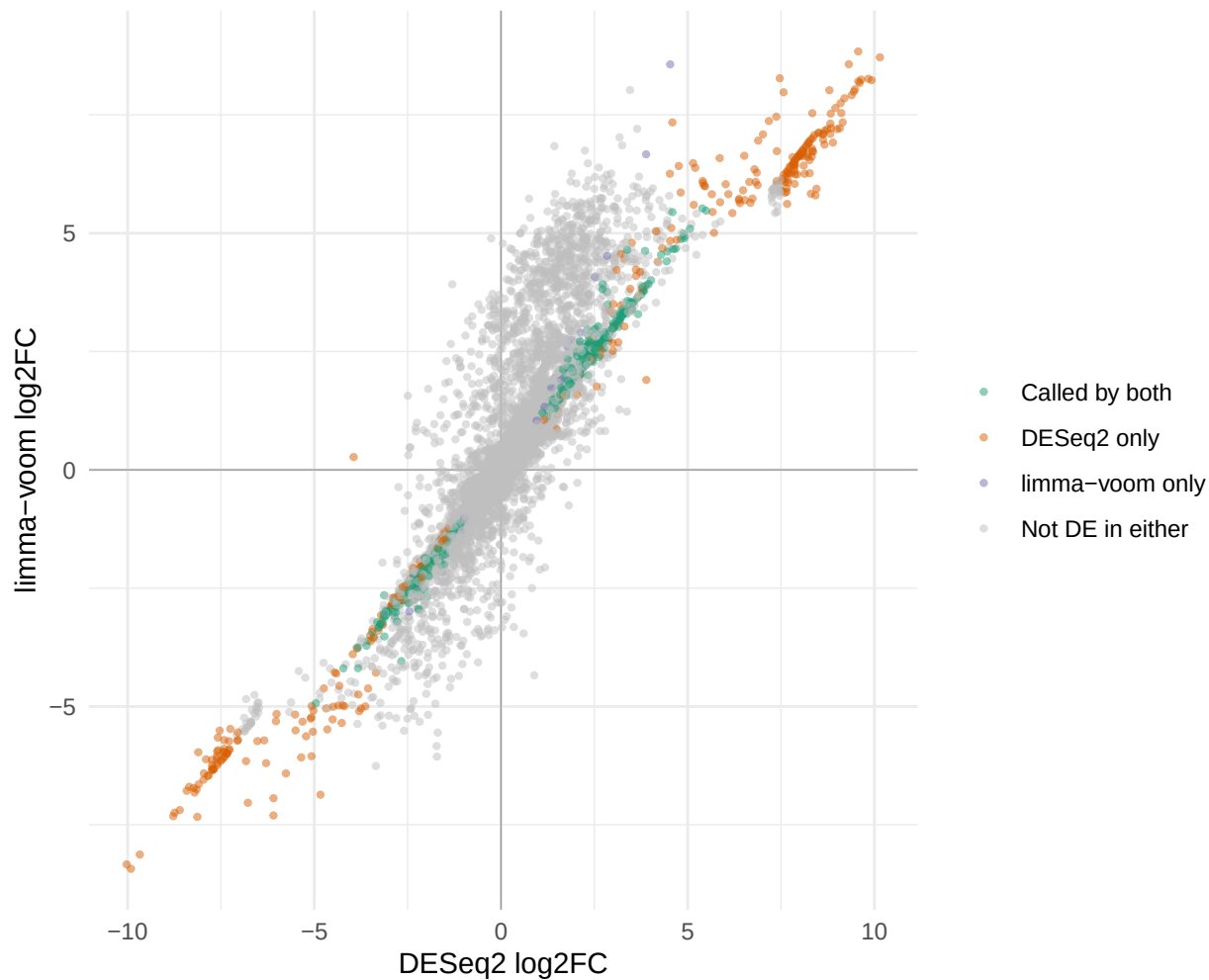
RNA DESeq2 vs limma-voom Concordance ( r = 0.901 )
