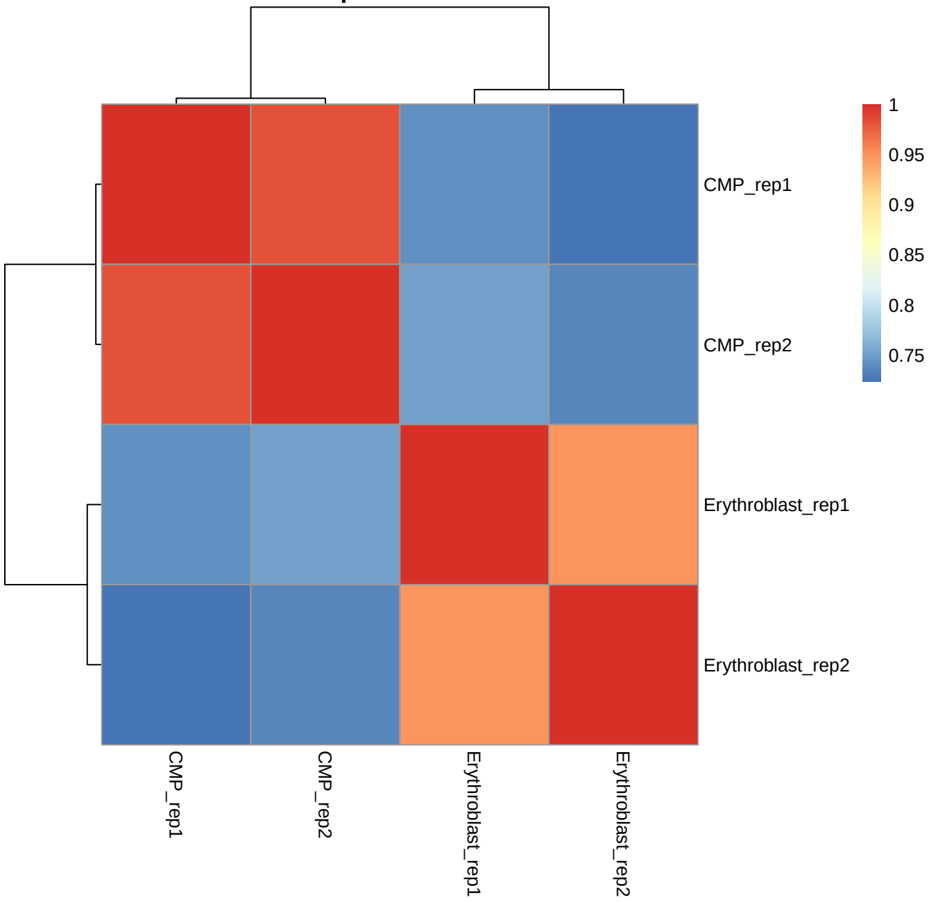
Sample Correlation
