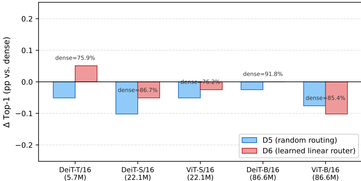
Cross-backbone accuracy retention (Imagenette, E = 4 , N = 200 , seed 42)
