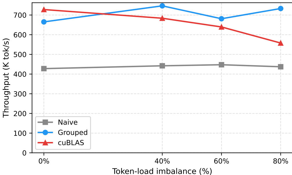
Dispatch throughput vs. load imbalance ( B = 8 , T = 1568 , E = 4 , GTX 960)
