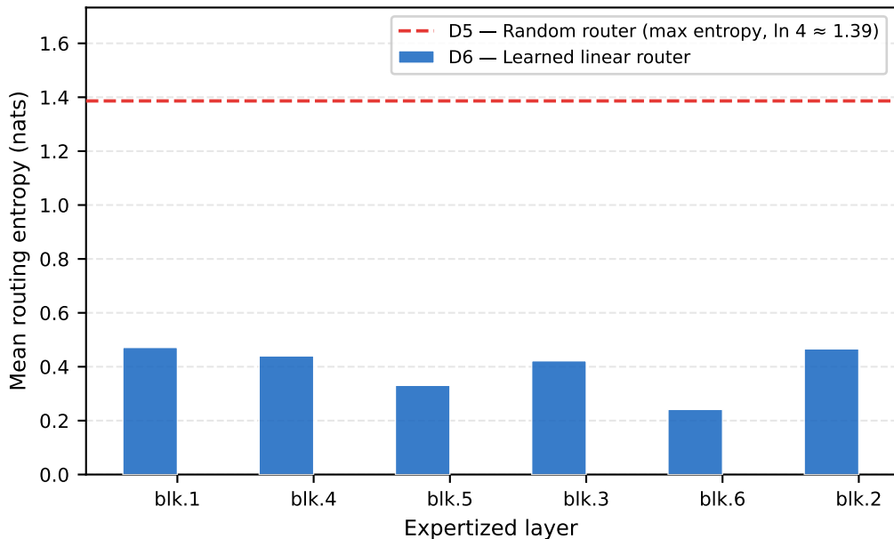
Per-layer routing entropy: D5 (random) vs D6 (learned)
