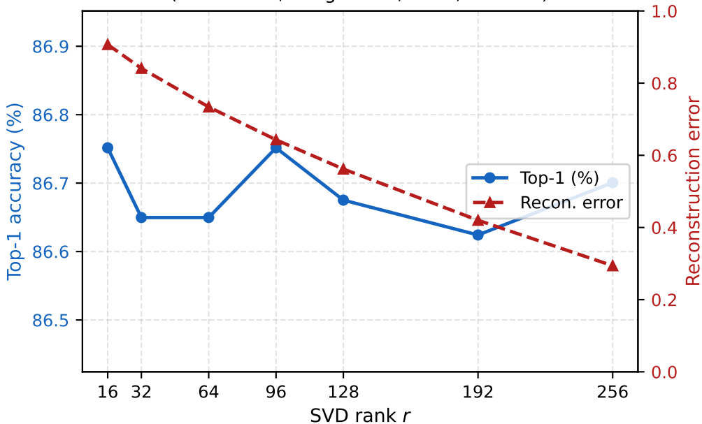
SVD rank vs. accuracy and reconstruction error (DeiT-Small, Imagenette, E = 4 , seed 42)
