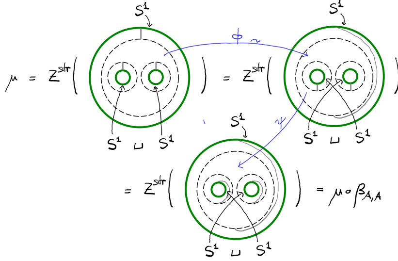
Figure 4.1: Demonstration of \mu = \mu \circ \beta_{A,A}
