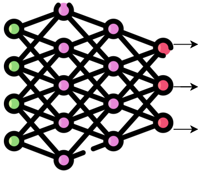
Neural network
