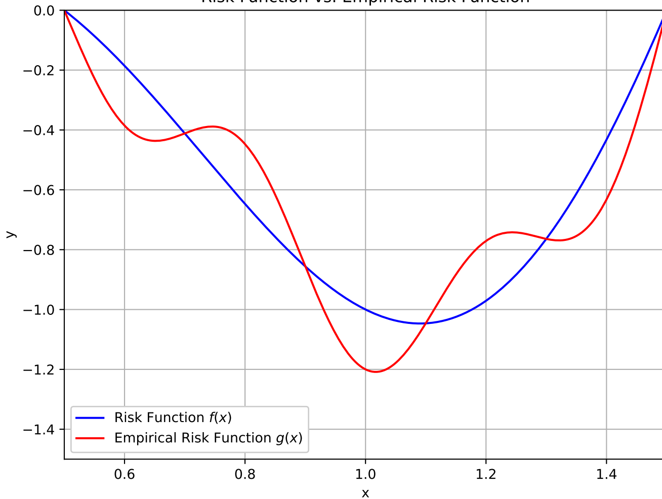
Risk Function vs. Empirical Risk Function
