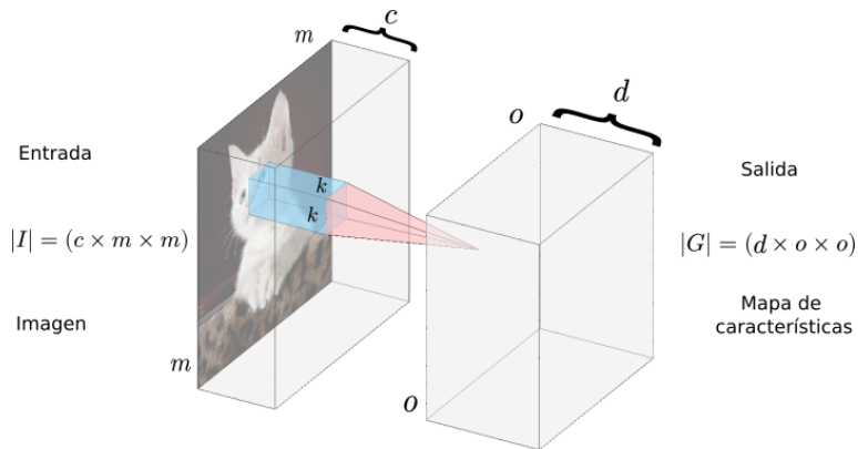
Figure: The depth of the feature map is the same as the number of applied kernels.
