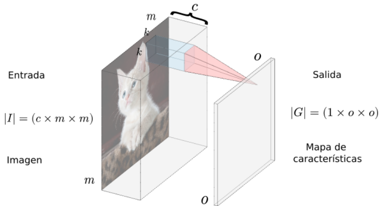
Figure: Convolution sizes of the multichannel convolution. The kernel's width and height are usually smaller than the input but the depth is the same than the input number of channels
