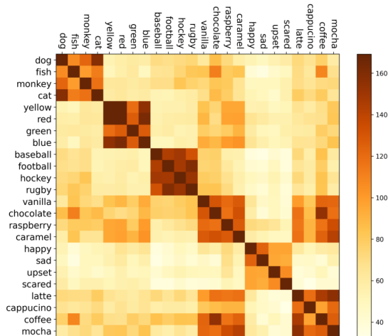
Figure: Word embedding correlation
