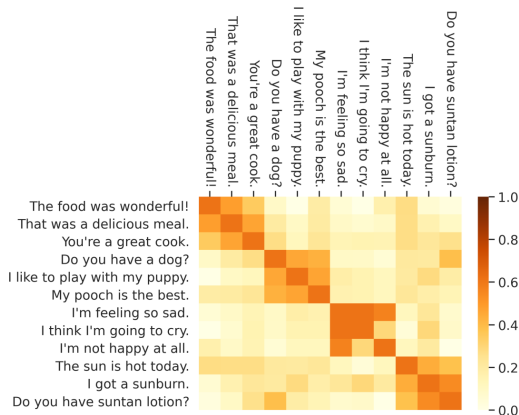
Figure: Correlation of embedded sentences
