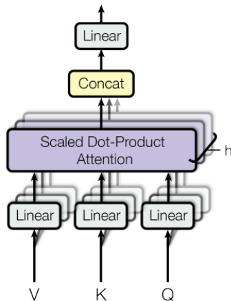
Figure: Multi-Head Attention consists of several attention layers running in parallel
