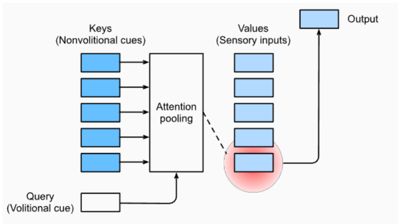
Figure: Attention mechanisms bias selection over values
