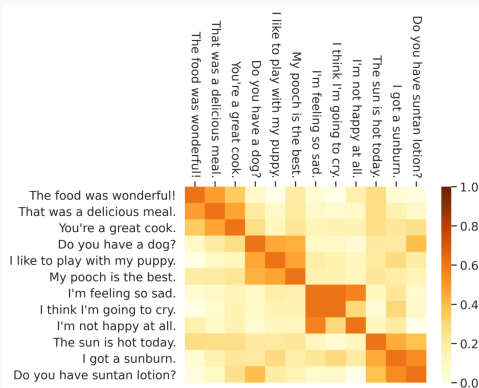
Figure 4: Correlation of embedded sentences
