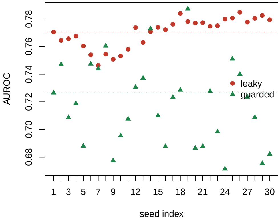
Per-seed AUROC (30 seeds)
