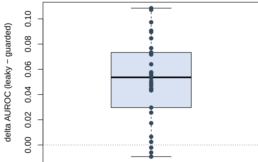
Leakage gap across seeds
