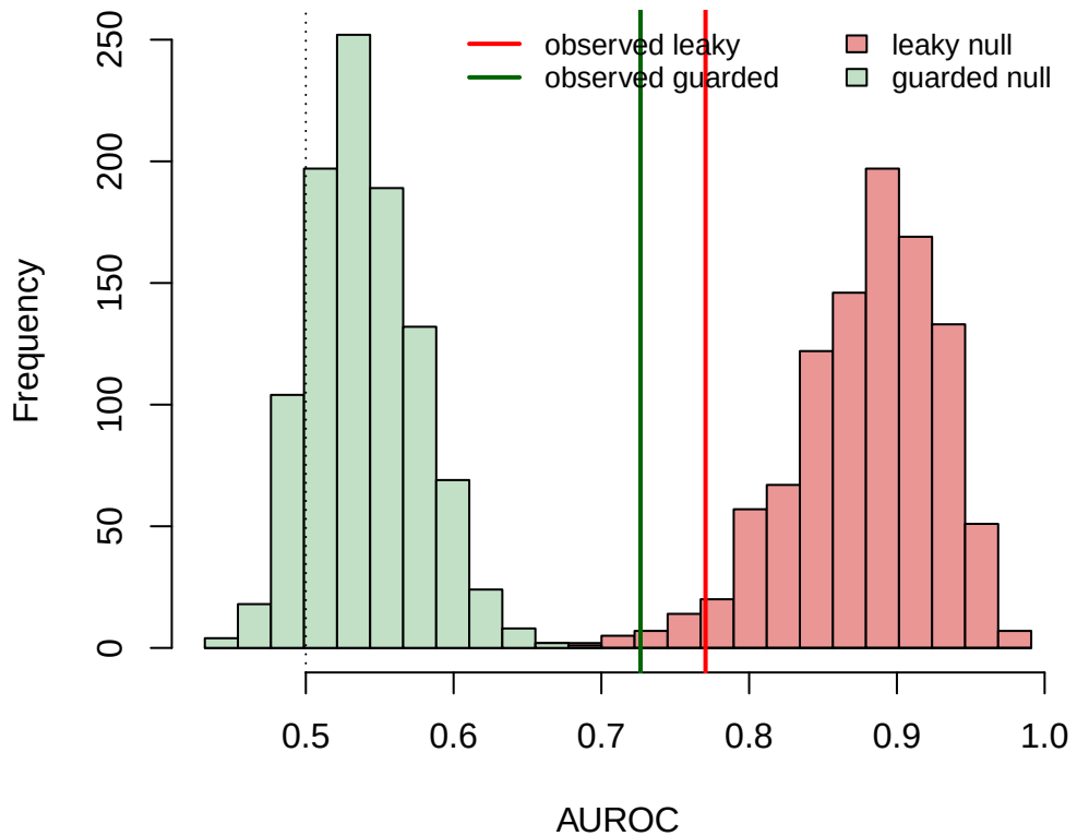
Null AUROC under shuffled labels
