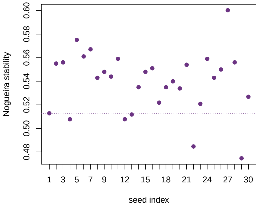
Per-seed Nogueira stability
